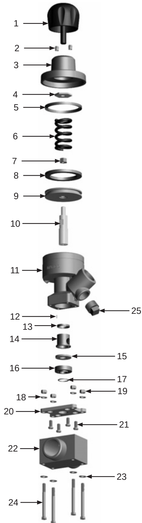
Figure 9: Blastmaster® Maxum III Abrasive Metering Valve — Tungsten Carbide Sleeve — 2”
